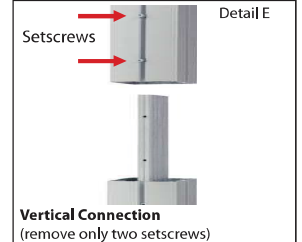
Vertical Connection (remove only two setscrews)
