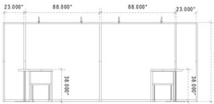
Magellan Miracle General Dimensions
